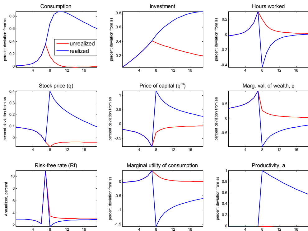
Figure 2. Impulse responses to a \eta shock to future TFP, E_t \{a_{t+8}\} .
