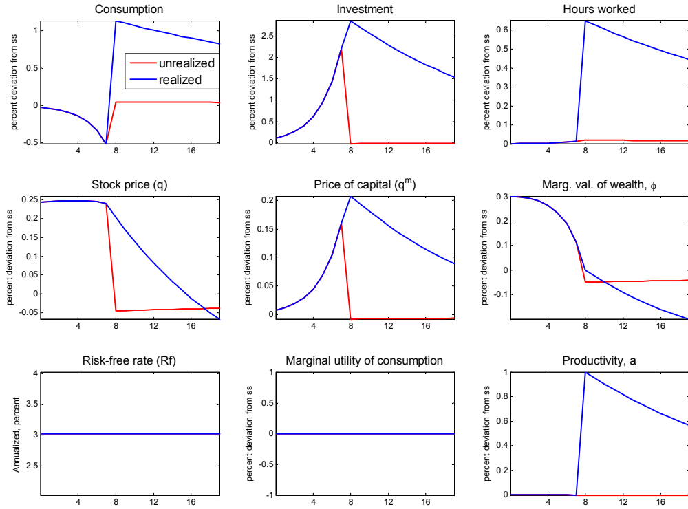
Figure 3. Impulse responses to a \eta shock to expected future TFP, E_t \{a_{t+8}\} . Setup with risk-neutrality and “level” adjustment costs.
