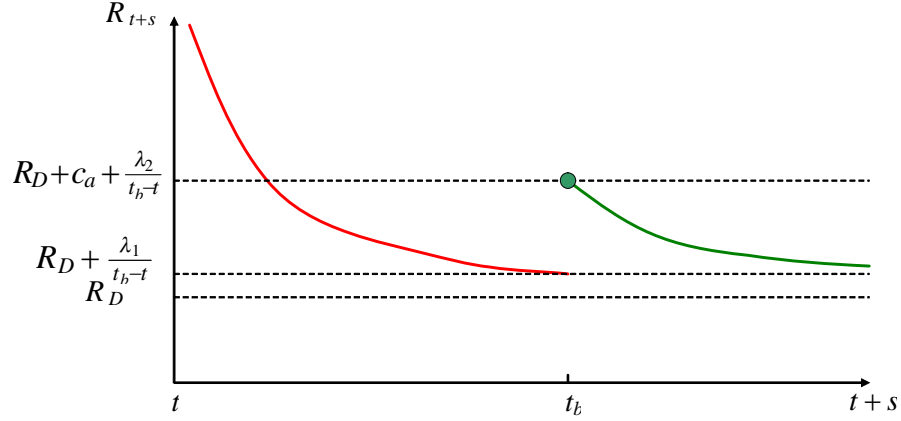
Figure 3: Time Path of the Discount Rate R_{t+s} in (12)
