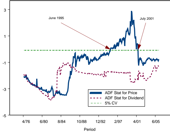
Figure 4: Time Series of ADF_r t -statistic for the Logarithmic Real Nasdaq Price and the Logarithmic Real Nasdaq Dividend ( r_0 = 0.1 ) from May 1976 to June 2005. ADF_r t -statistic is obtained from the forward recursive regression with the first observation in February 1973.
